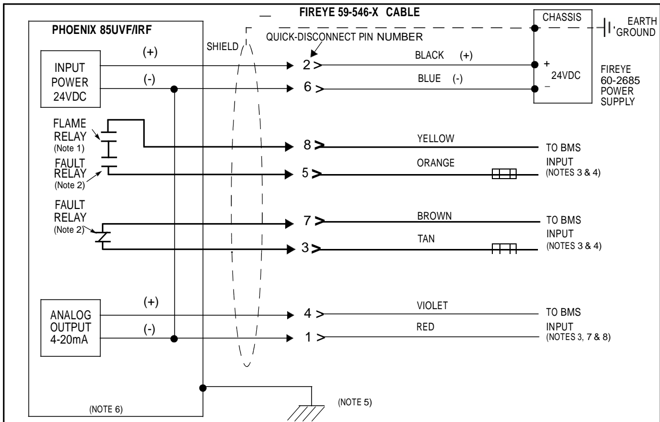
FIGURE 6. WIRING DIAGRAM
