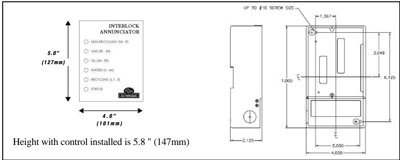
FIGURE 1. DIMENSIONS
