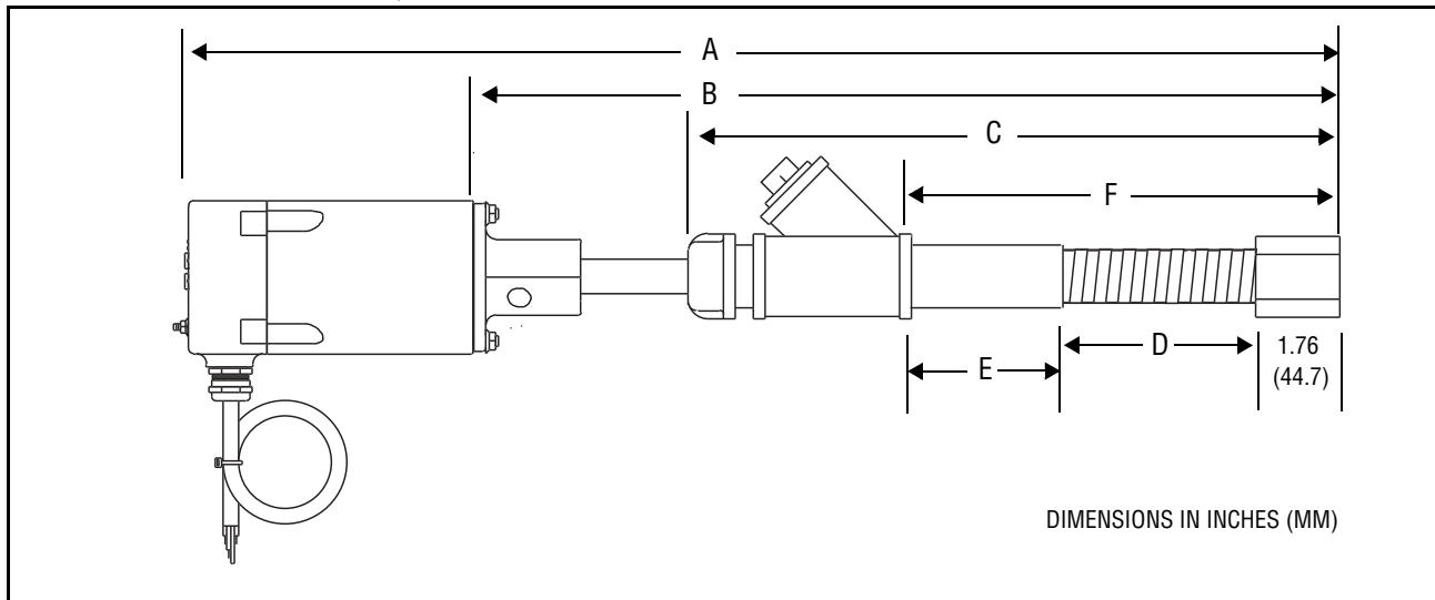
FIGURE 1. DIMENSIONS, SCANNER WITH FIBER OPTIC INNER AND OUTER CARRIERS
