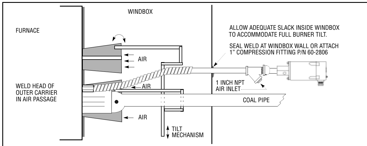
FIGURE 5. ALTERNATE LOCATION OF FIBER OPTIC ASSEMBLY
