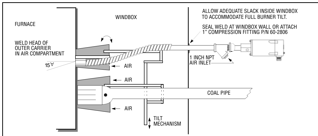
FIGURE 5. ALTERNATE LOCATION OF FIBER OPTIC ASSEMBLY
